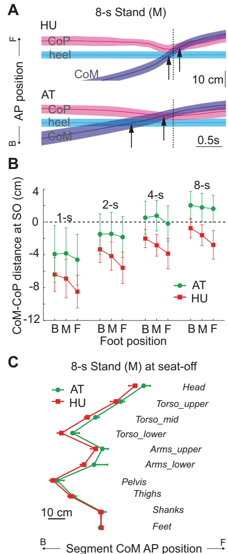
Fig. 4. Bipedal balance. A : trajectories of horizontal CoM (blue), combined-feet CoP (pink) and heel position (cyan) for the 8-s middle (M) foot condition for both groups. Shaded areas indicate 95% CI. Black arrows demarcate when the CoM reaches the heel and CoP, achieving forward balance. Note that at SO (dotted line) the CoM was anterior to the heel and CoP for AT, but only the heel for HU. B : CoM-CoP distance at SO ( \pm SD). Positive values indicate the CoM was anterior to the CoP. Note that AT achieved a more forward CoM position than HU by SO for all conditions. Static stability at SO (i.e., CoM-CoP > 0) only occurred for the AT group (4- and 8-s conditions). C : AP positions of the segmental mass centroids at SO, relative to CoP, for the 8-s middle condition. The vertical axis is arranged to approximate vertical segmental position. The arms were placed just above the pelvis to avoid overlapping with the torso. AT's anterior whole body CoM at SO was largely due to more anterior upper body segments.
