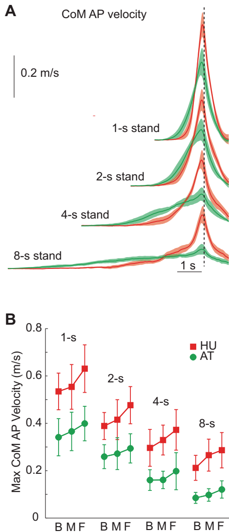
Fig. 3. Center-of-mass (CoM) velocity ( V_{CoM} ). A : time course of V_{CoM} for HU (red) and AT (green) while standing up from the middle foot position at each speed. The shaded area indicates 95% CI, and the dotted line indicates SO. B : maximal horizontal V_{CoM} across all movement conditions. HU had a greater maximal velocity than AT for all conditions. Note that for the slower conditions, HU had a low initial velocity but large increase just before SO, thereby violating the task instruction to stand up at a uniform speed. AP, anteroposterior.
