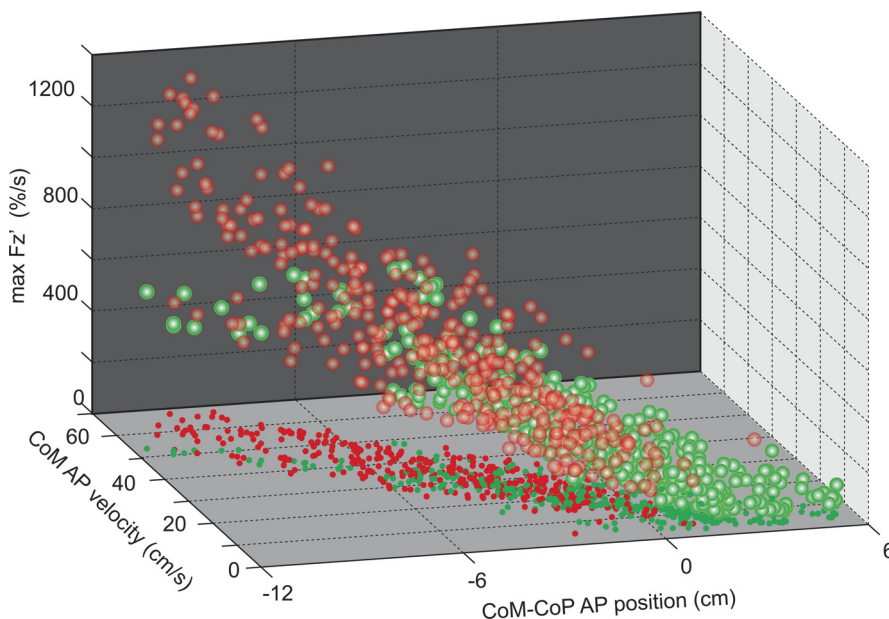
Fig. 6. Interrelation between weight shift, V_{CoM} and bipedal balance. Each subject's condition averages for F_z^i max, V_{CoM} at SO and CoM-center-of-pressure (CoP) distance at SO. Red dots with white center indicate data from HU, and green dots with white center indicate AT. Smaller solid dots mark the projection of data onto the horizontal plane. For each group, data for the slowest conditions are toward the front lower right and fastest conditions are in the rear upper left. The majority of variance across condition and group (91.5%) is described by a single principle component revealing a strong relationship between these three variables. However, AT data are shifted along this component toward a further forward CoM, slower V_{CoM} and lower F_z^i max relative to HU.
